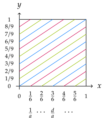
FIGURE 8.2: The pullback in the case a = 6 and b = 9 (so d = 3 ). The square represents the unit square and we've drawn the solution to ax = by \pmod{1} , corresponding to z^a = w^b when z = e^{2\pi i x} and w = e^{2\pi i y} . On the torus S^1 \times S^1 , the solution consists of three circles.
