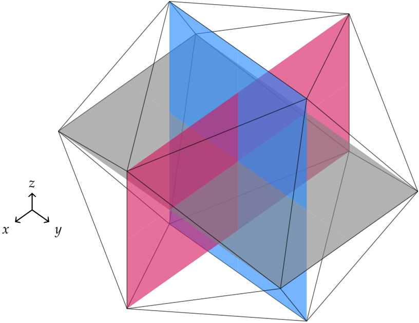
FIGURE 14.1: Icosahedron with its golden rectangles.
