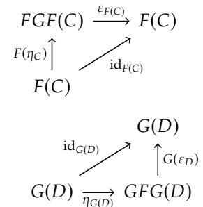
FIGURE 6.2: Triangle laws for an adjunction F \dashv G .
