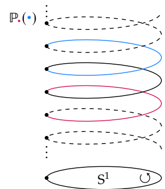
FIGURE 3.5: For the fiber of the universal set bundle, \mathbb{P}.\bullet \equiv (\bullet = \bullet) , we increase the winding number (in blue) along \cup , and we decrease it when we transport the starting point (in red) in the same way.
