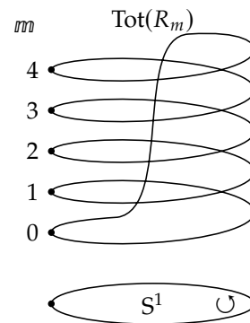
FIGURE 3.7: The m^{\text{th}} power bundle for m = 5 .
