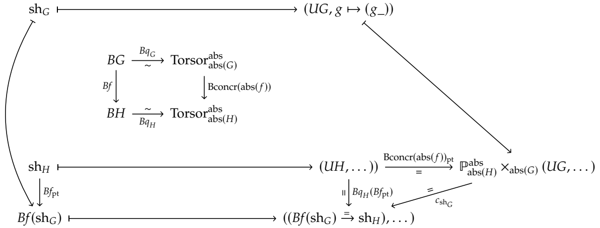
Figure 7.1: Commuting inner square of maps and lower right triangle of pointing paths.
